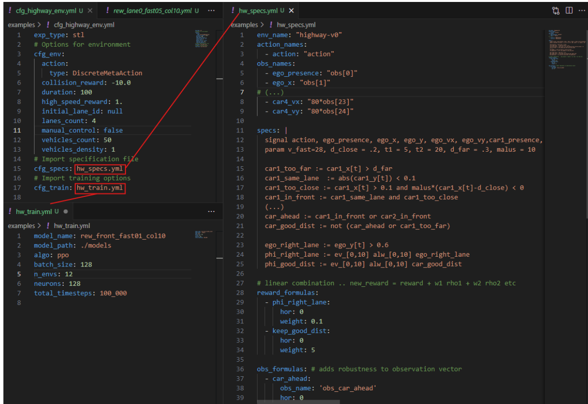
Figure 1: Configuration files for the highway-env environment. At the top level (cfg_highway_env.yml, there are three main sections for environment options, specifications and training options. These sections can be included directly, or imported from other files. When training occurs, the configuration file is flattened into a single file and copied along with the trained model so that the training can be reproduced more easily.
